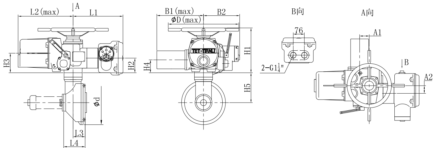
SMC-03. IN带BA外形尺寸
